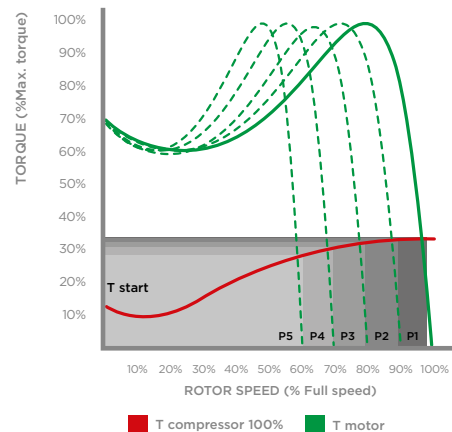
VSD CONTROL
