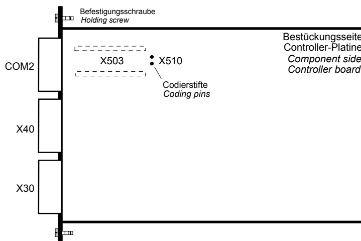
Optionsplatine RP 422 Option board RP 422
